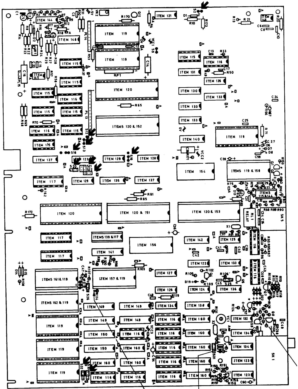
PCB Links inside the BBC Microcomputer
